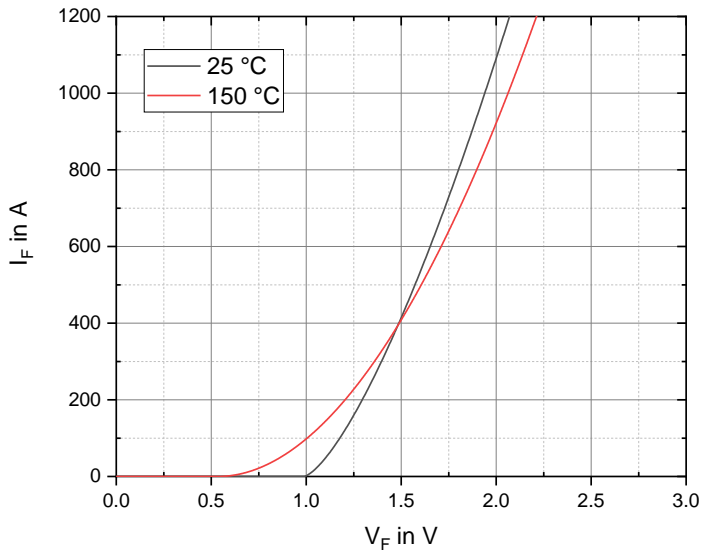
Fig. 3 Typical diode forward characteristics, chip level
