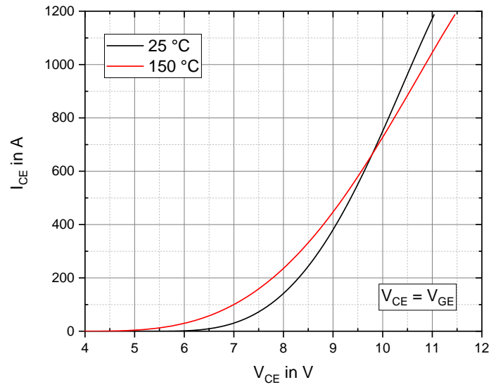
Fig. 2 Typical transfer characteristics, chip level
